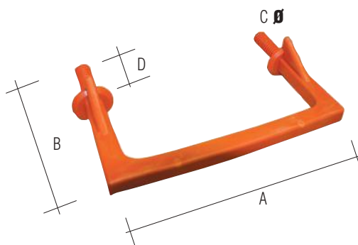
GRADINO IN ACCIAIO RIVESTITO PVC STEEL COATED STEEP WITH PVC
